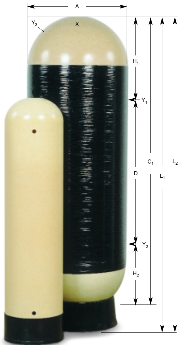
Standard Vessel Openings
